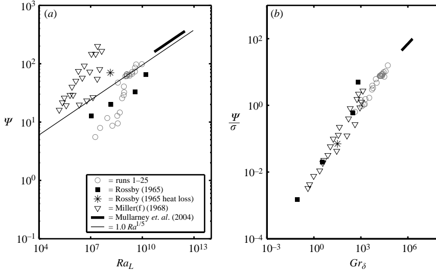
FIGURE 15. (a) The dependence of overturning rate on Rayleigh number for all the experimental results. (b) The relationship between \Psi/\sigma and the Grashof number for this study (runs 1–25) and previous studies. The star indicates the special case with heat loss in Rossby’s experiments.
